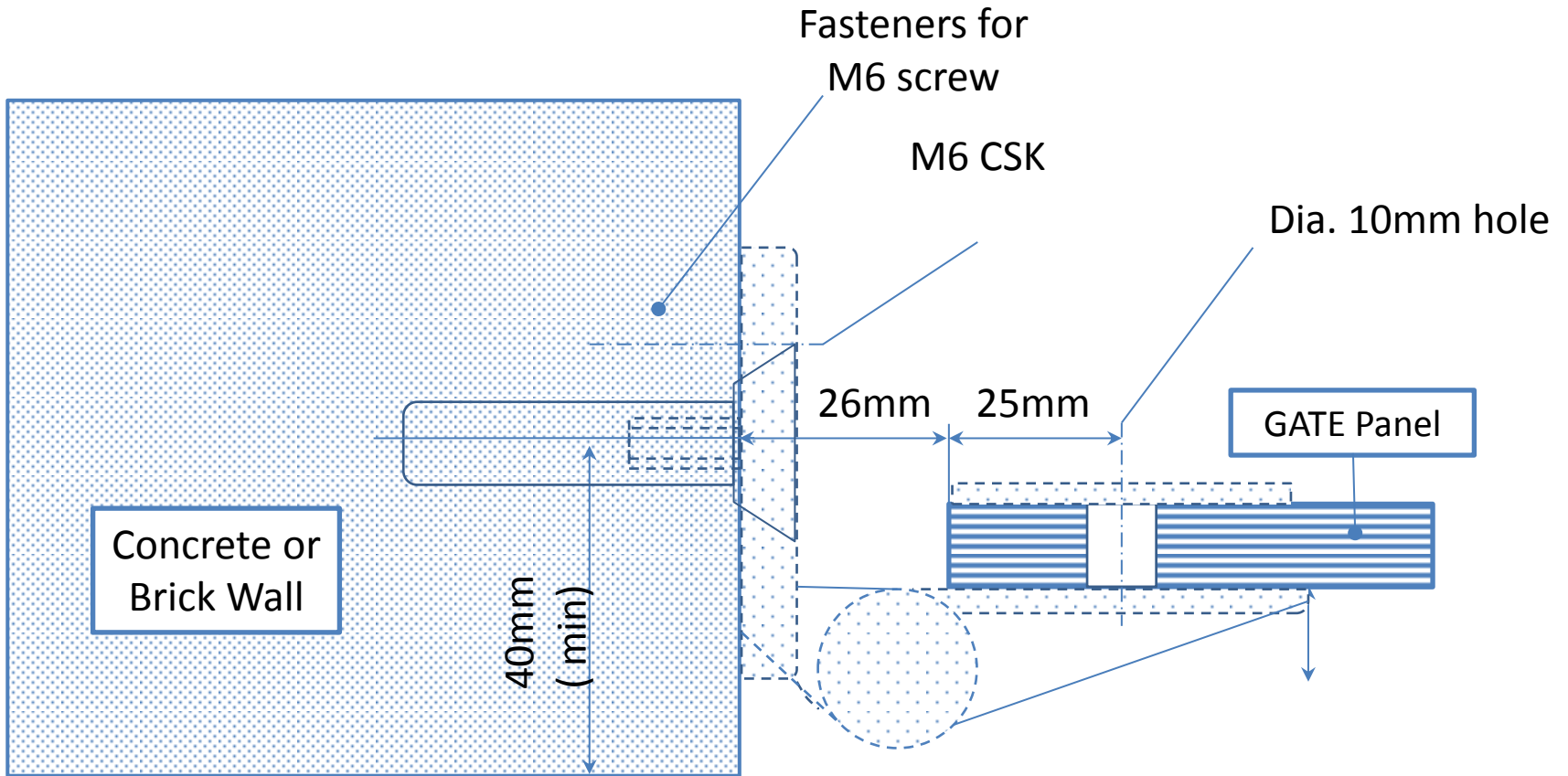
PLAN of Detail X
